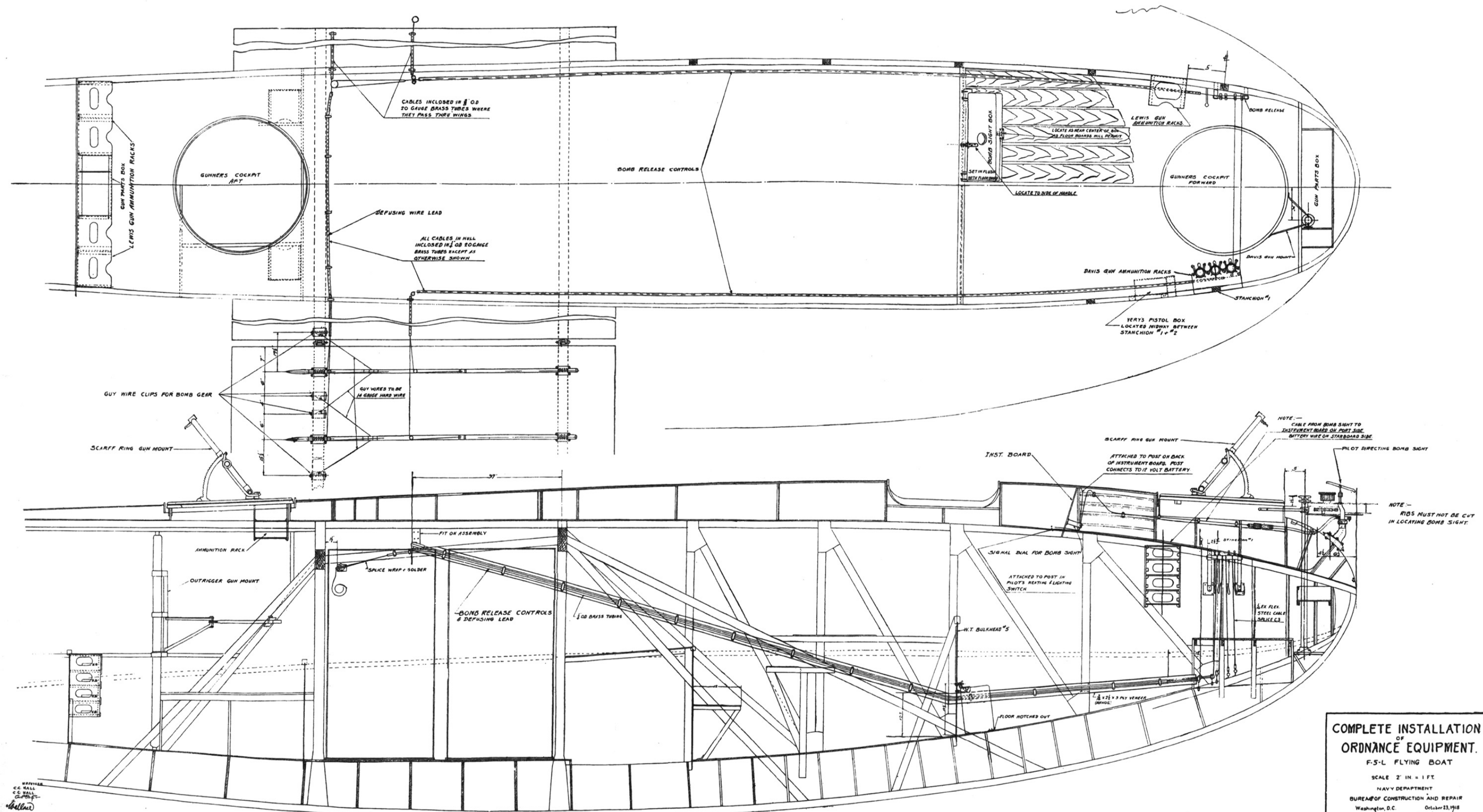
FIG. 57.—ORDNANCE INSTALLATION.
