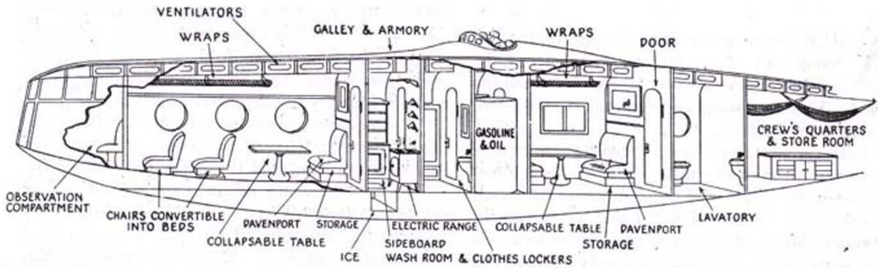
Cross section of the Aeromarine flying boat "Polar Bear" built to make a hunting trip to the Arctic Circle.
